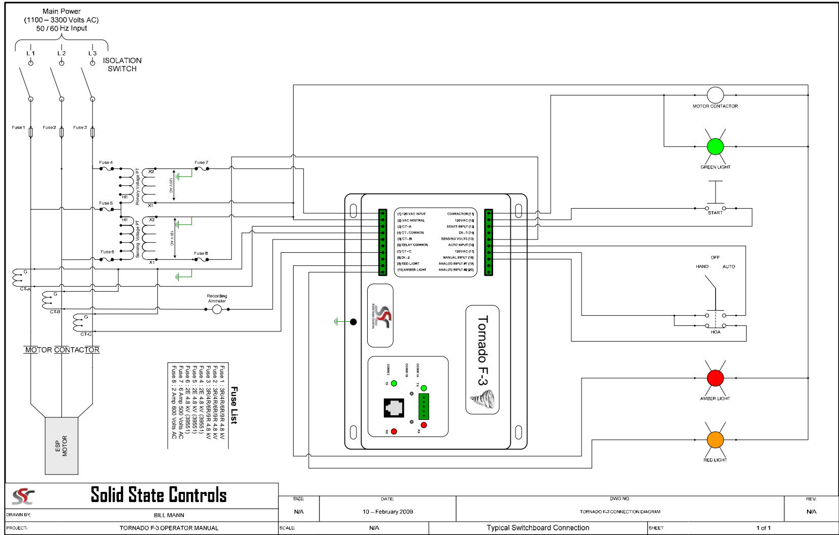
Figure 4 - Typical Switch Board Connection
