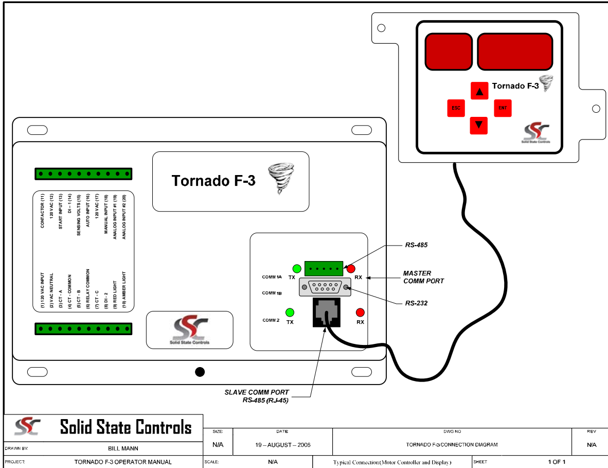
Figure 3 - Typical Connection
