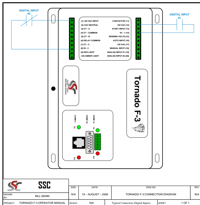
Figure 5 - Typical Digital Inputs
