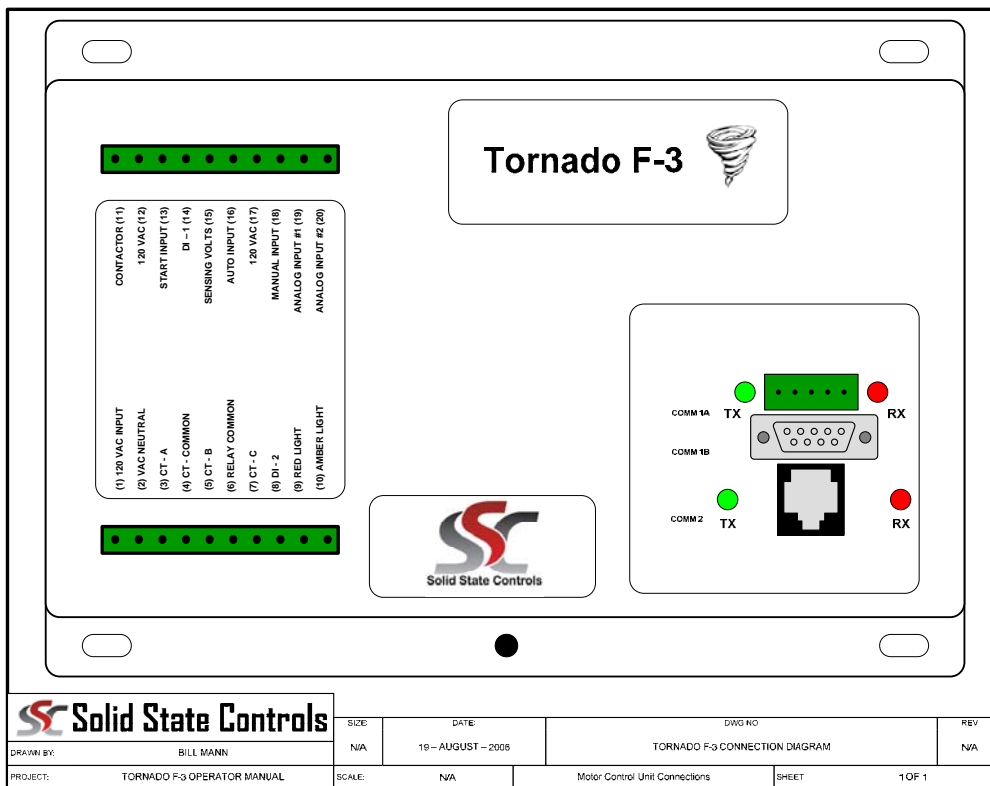
Figure 1- Motor Controller Unit Connection
